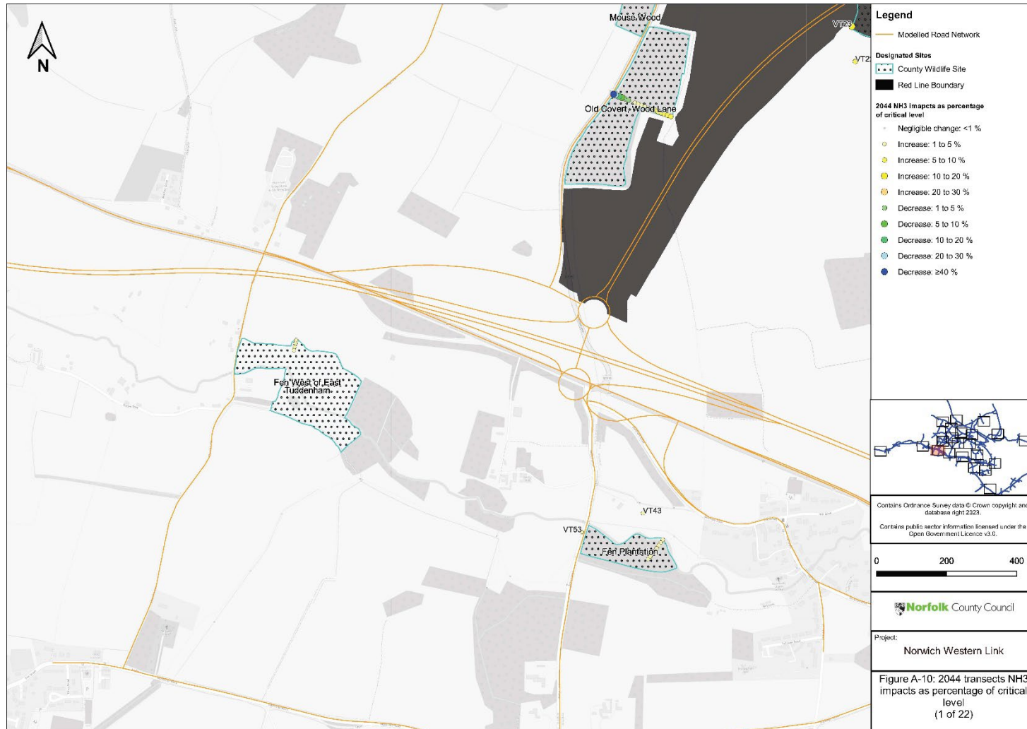
Figure A 10 2044 Transect NH3 Impacts as percentage of critical level
